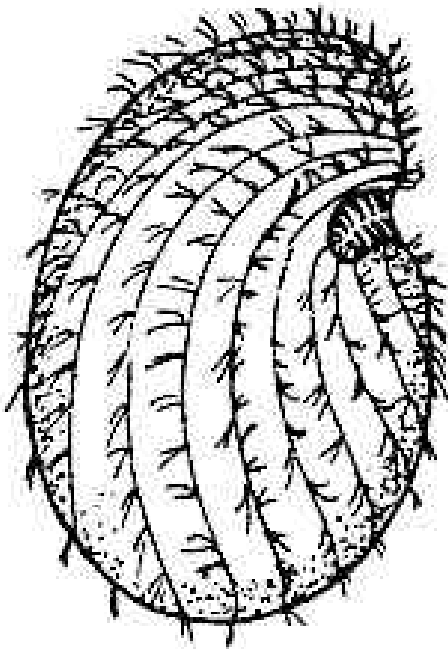
Colopoda (40-110 microns)
